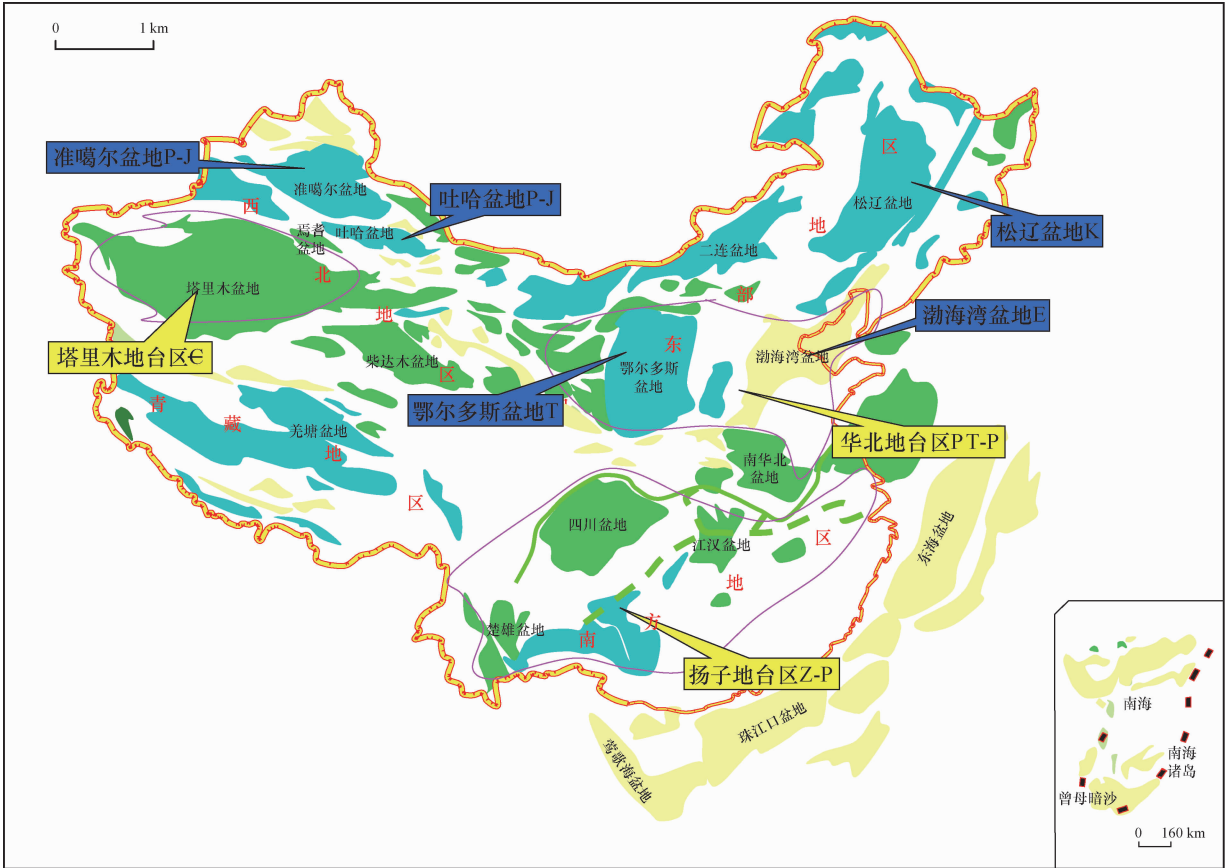
图4 中国页岩气有利勘探领域示意图 Fig.4 Sketch map showing the play fairways of shale gas in China
